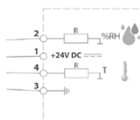
Analogica 4-20 mA
